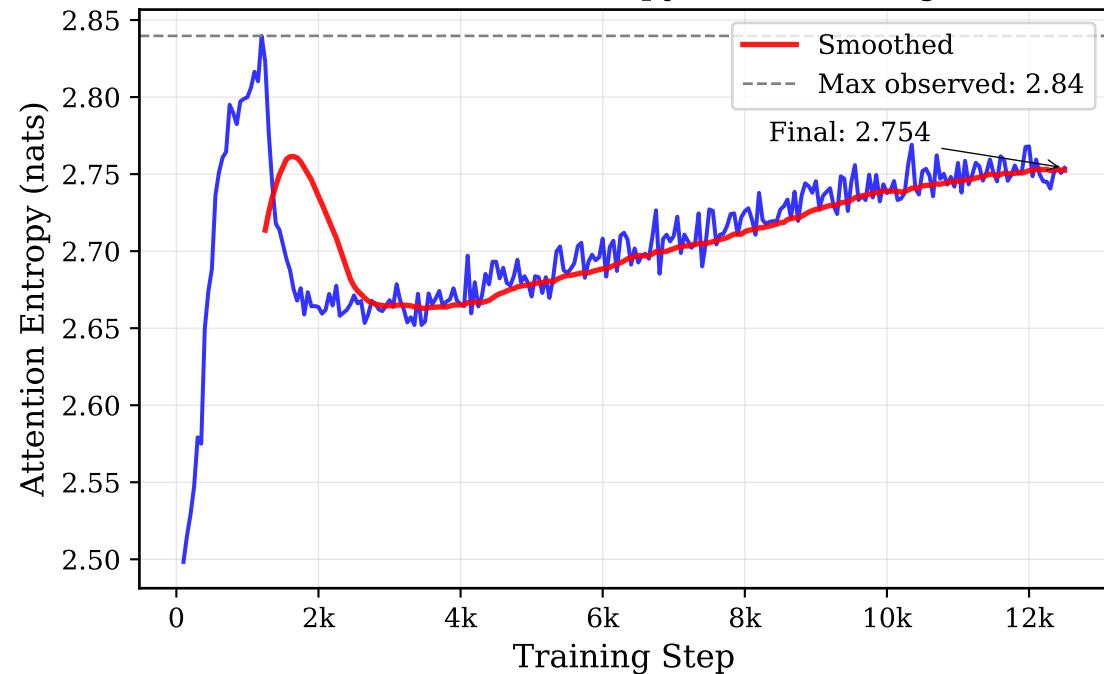
(a) Attention Entropy Over Training
